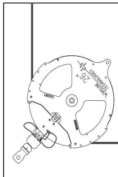
Safe Line Tension for 90-Degree Deflection Figure 4
